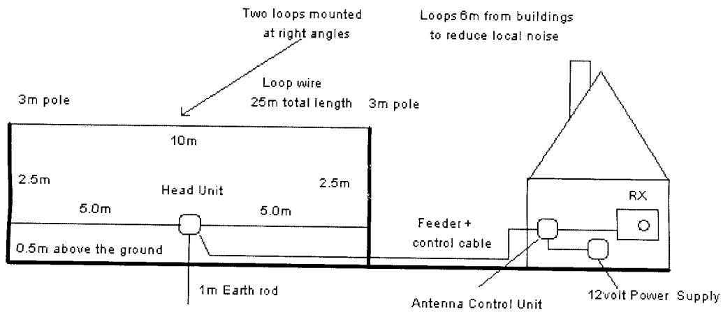
FIGURE 2 ALTERNATIVE INSTALLATION
