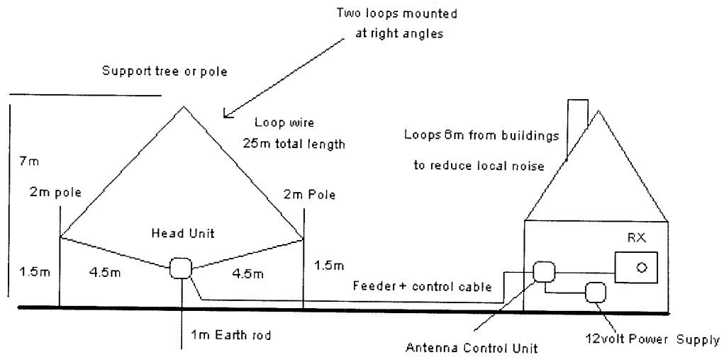
FIGURE 1 TYPICAL INSTALLATION
