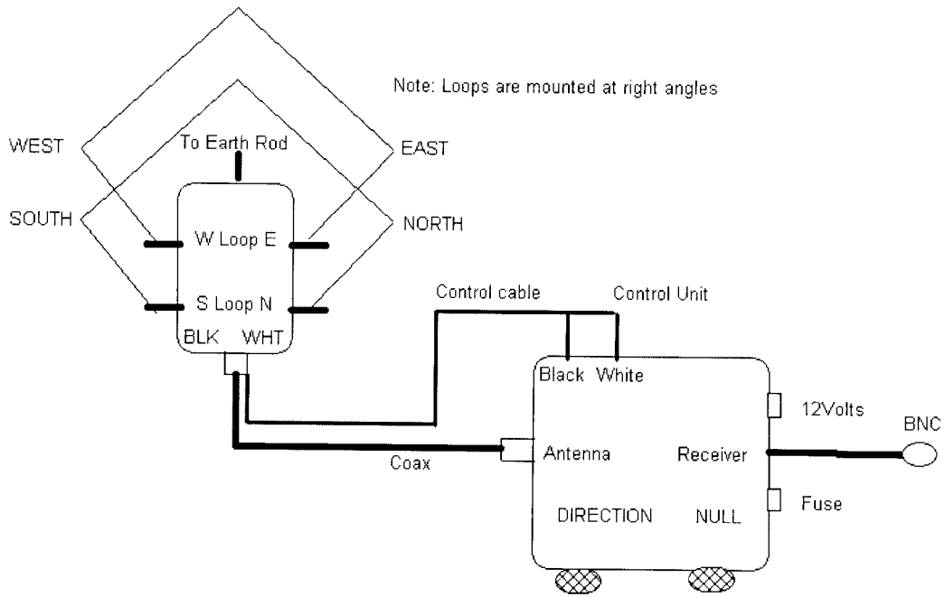
FIGURE 3 HEAD UNIT AND CONTROL UNIT WIRING DIAGRAM
